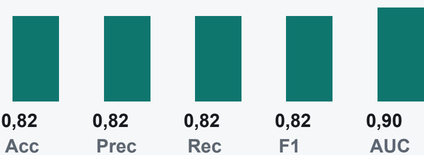
Embeddings + RL
