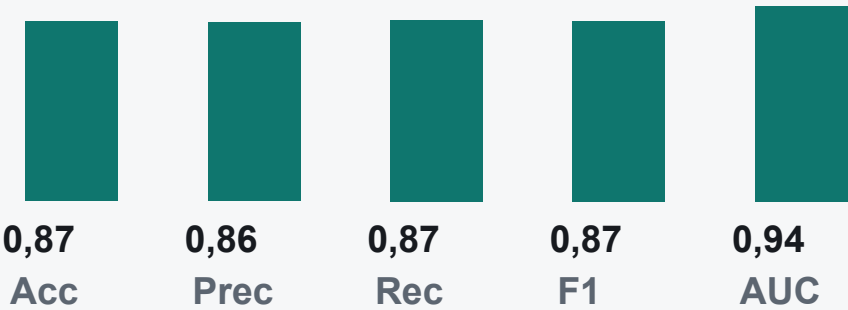
Stacking
