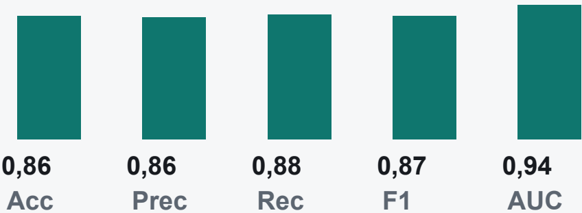
LightGBM
