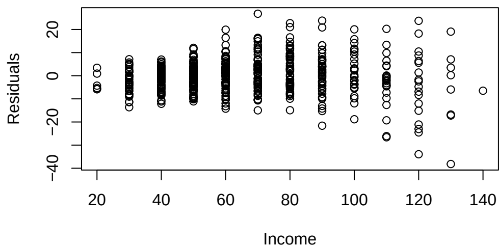
Residuals vs Income
