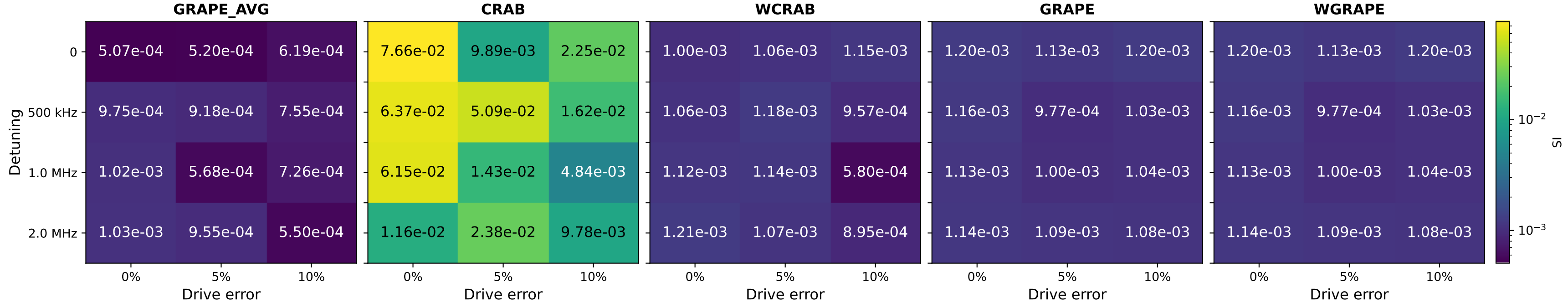
Minimum Secret Independence under Detuning and Drive-Amplitude Errors N_{ts} = 40, \lambda = 0.05
