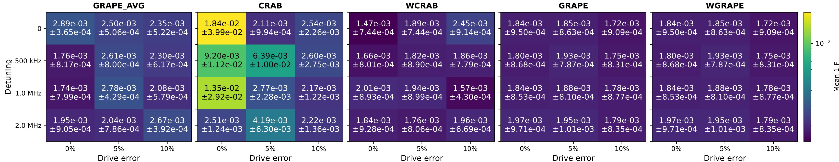
Mean State Infidelity of the minimum-SI Solution under Detuning and Drive-Amplitude Errors N_{ts} = 40, \lambda = 0.05
