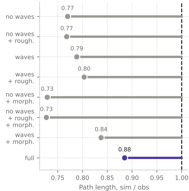
(a) How far the particles went
