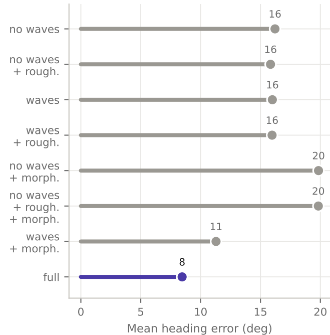
(c) Which way they went
