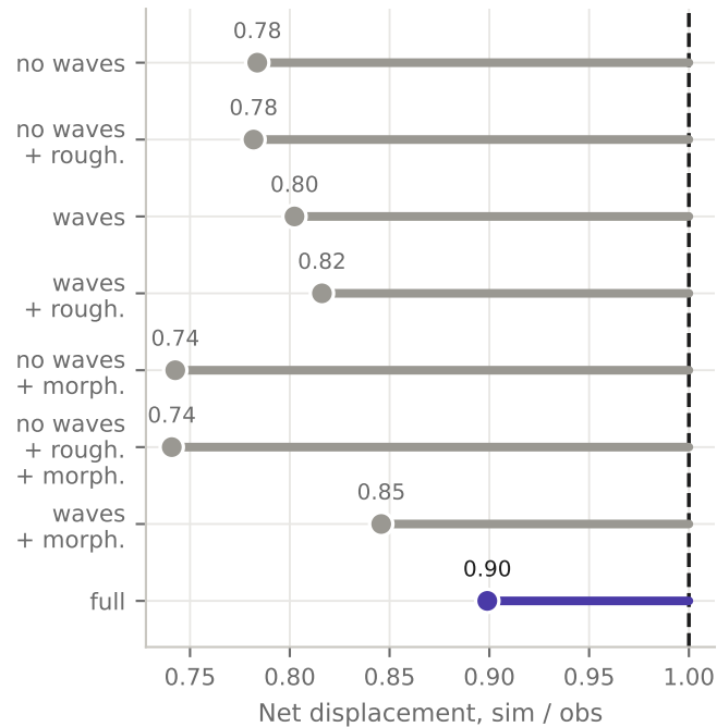
(b) How far they ended up
