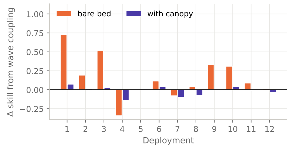
(b) Wave contrast on a mobile bed, by deployment
