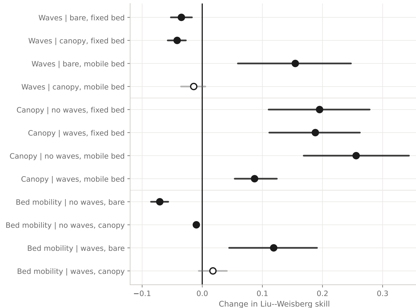
(a) Twelve single-factor contrasts, 95% bootstrap CI
