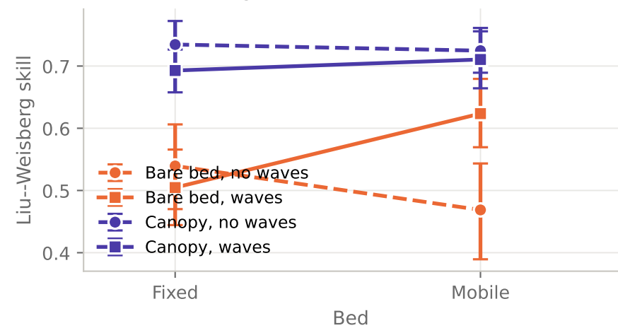
(c) Mean skill against bed treatment
