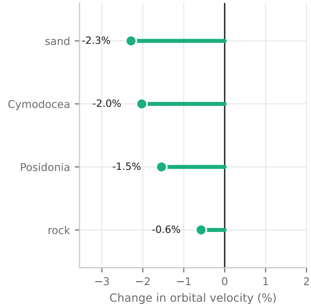
(c) Roughness effect on waves
