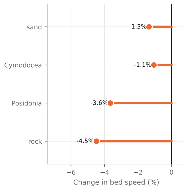
(b) Roughness effect, fixed bed
