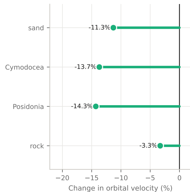
(c) Roughness effect on waves
