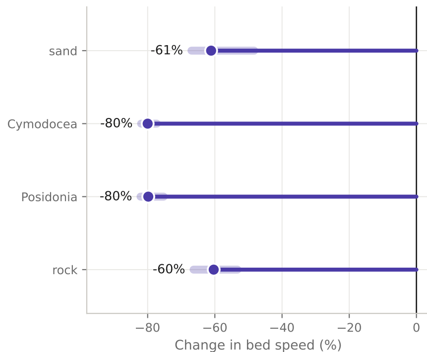
(c) Canopy effect on bed speed
