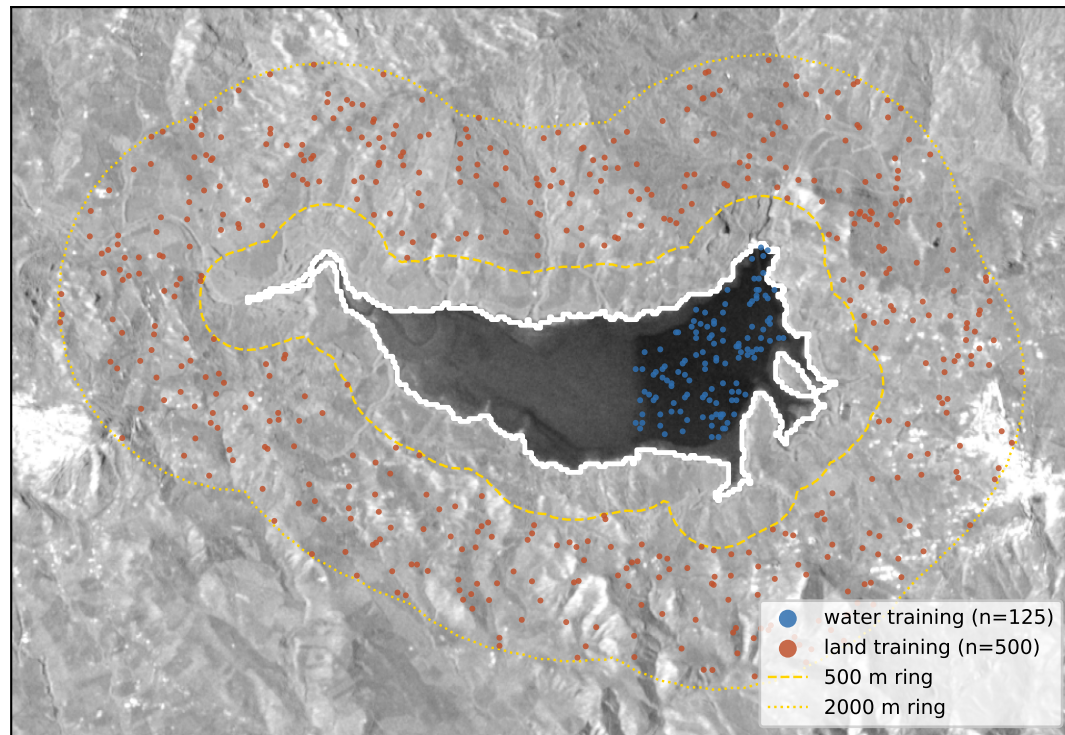
(a) SVM training samples JRC water occurrence + WorldCover land, 500-2000 m ring
