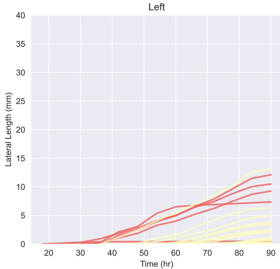
Lateral Lengths by Time (p35, setup:LL)
