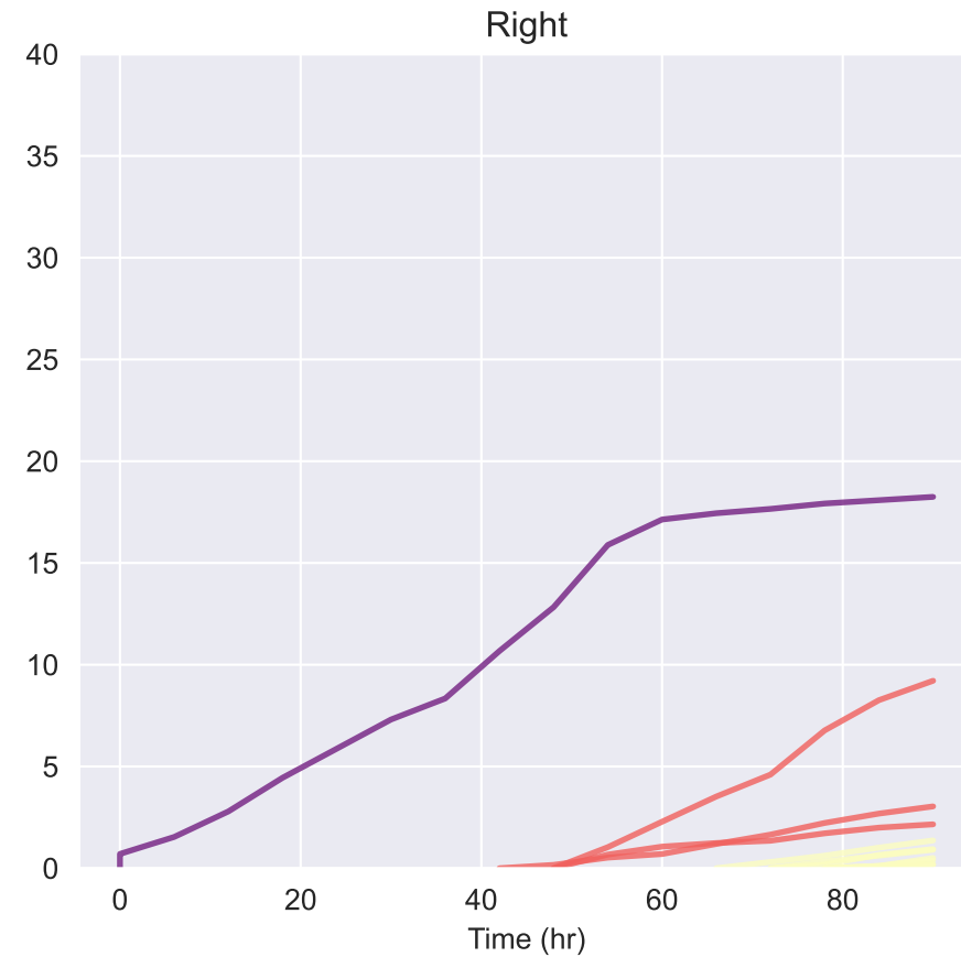
Lateral Lengths by Time (p35, setup:LL)
