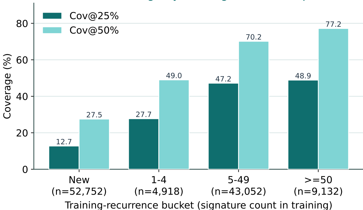
Meta+Cal coverage by training recurrence (panel b)
