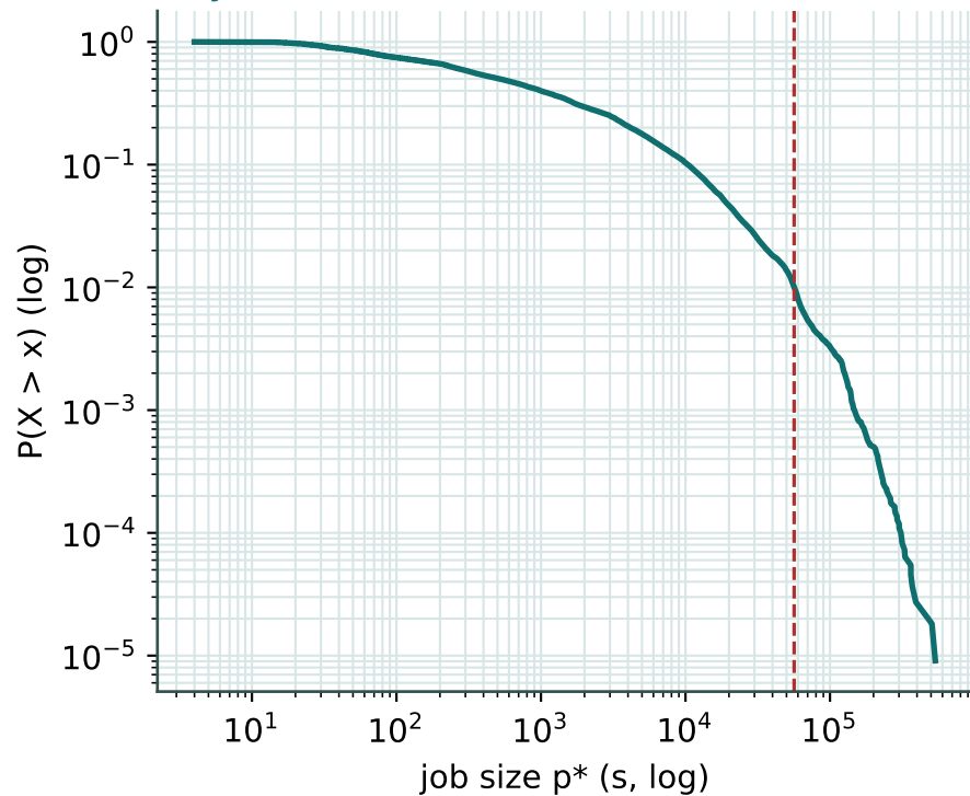
A. Heavy-tail CCDF (P99/P50 \approx 110x, max=535085s)
