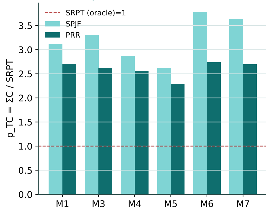
B. Competitive ratio vs SRPT (oracle)
