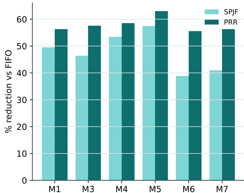
B. \Sigma C reduction vs FIFO (%)
