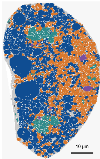
Neck connective cross-section (16 nm EM segmentation)
