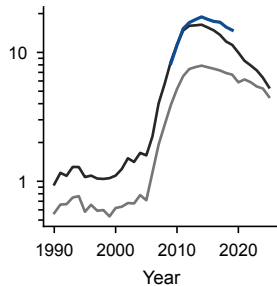
D Graphene
