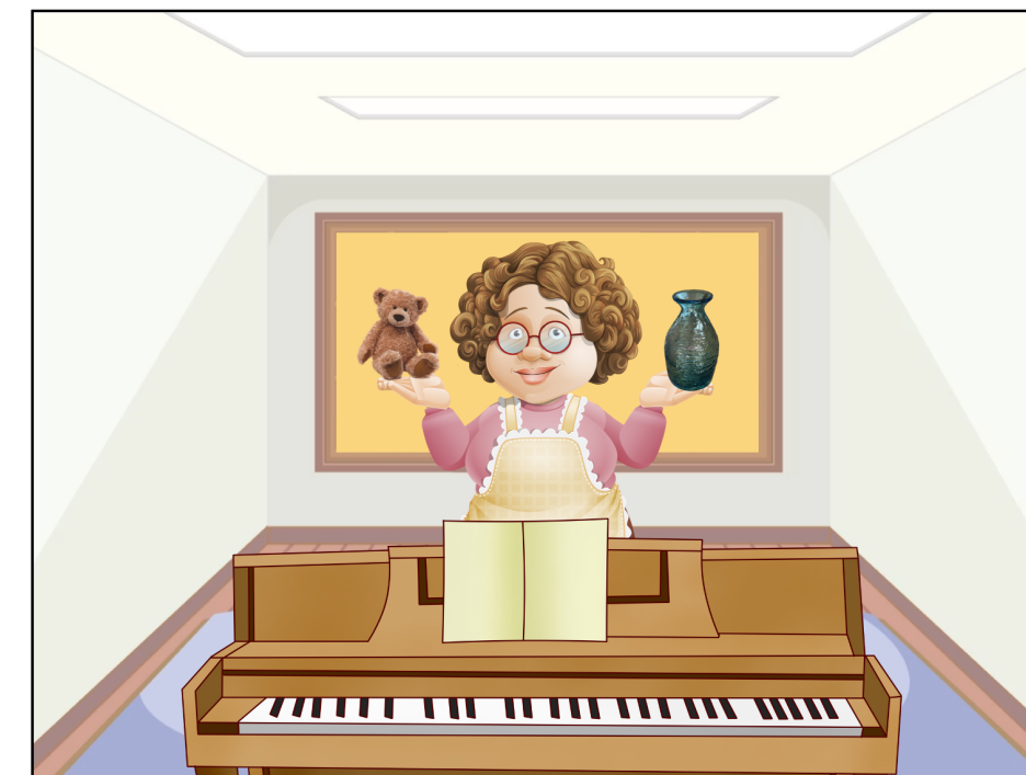
bear | vase
