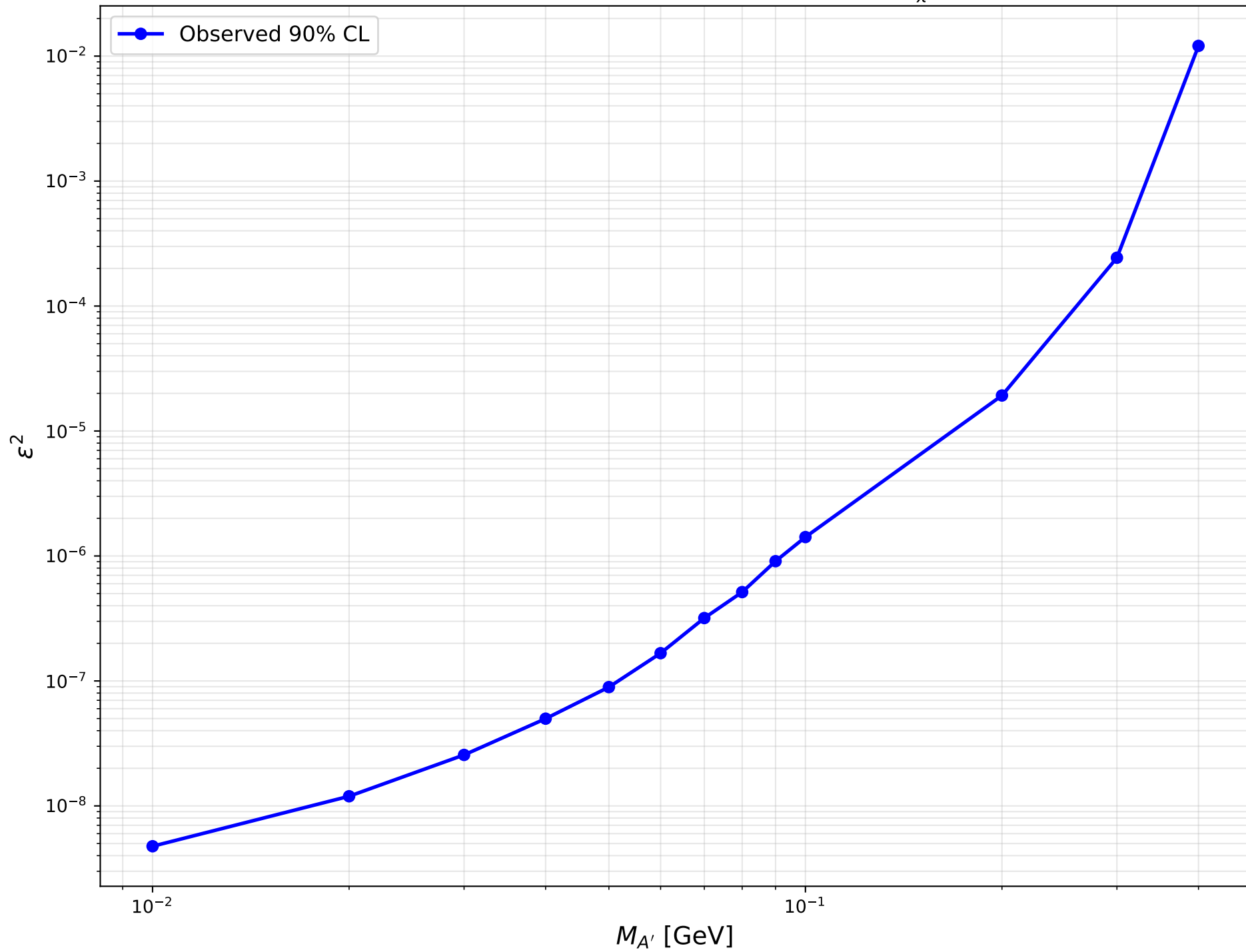
Dark Photon Sensitivity - Fermion DM ( \alpha_D = 0.1 , M_\chi/M_{A'} = 0.6 )
