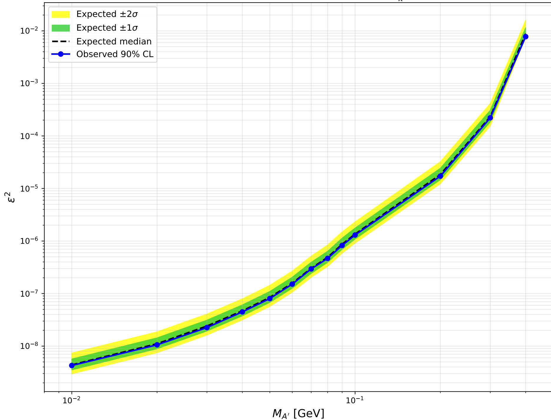
90% CL Upper Limits - Fermion DM ( \alpha_D = 0.1 , M_\chi/M_{A'} = 0.6 )
