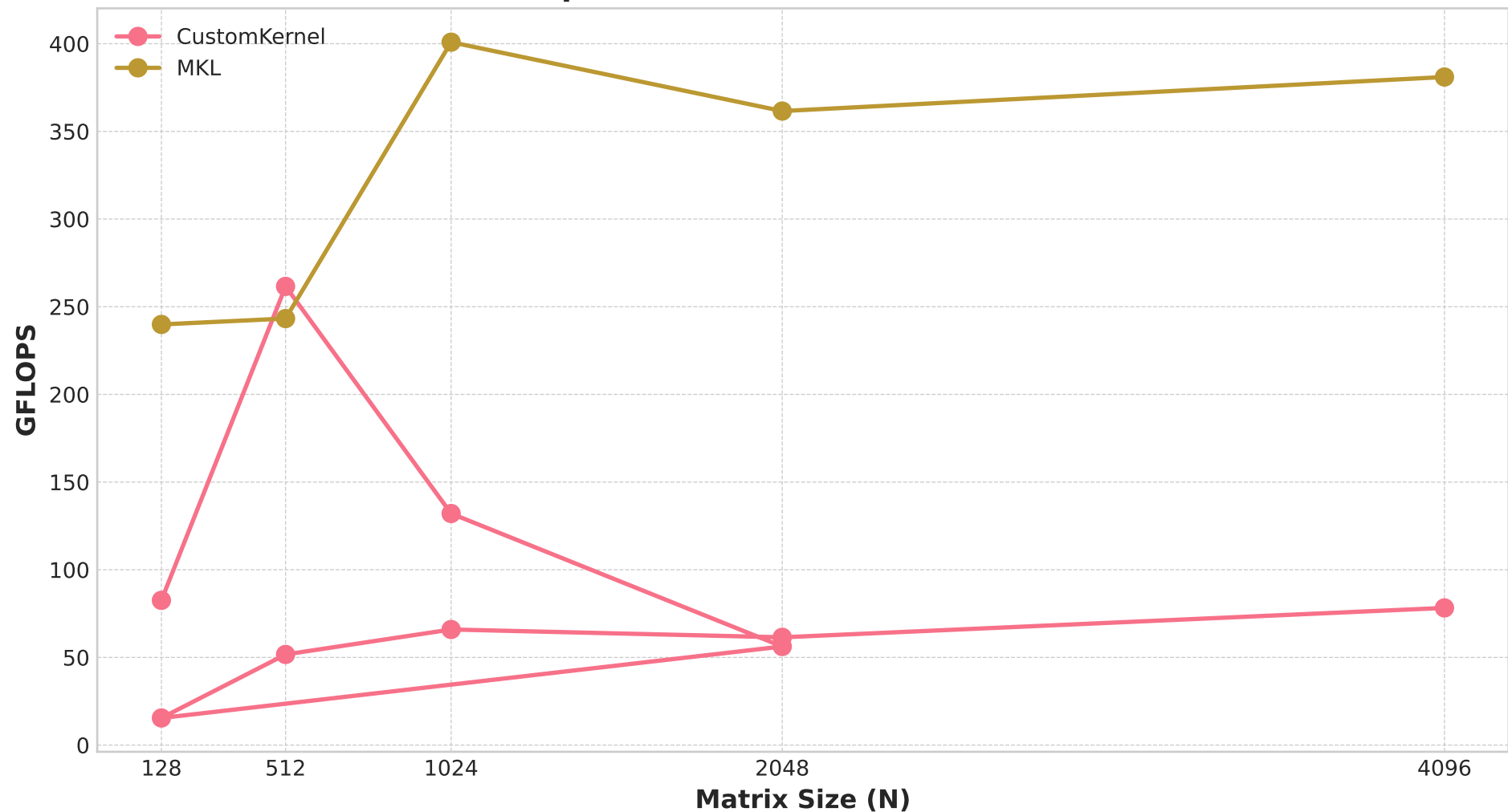
Performance Comparison: Custom Kernel vs MKL (OpenMP, AVX2/YMM, TSC-timed)
