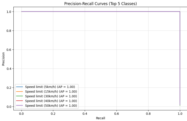
Figure 4. Precision-recall curves for the top five traffic sign classes, showing strong class-wise performance with average precision values close to 1.00.
