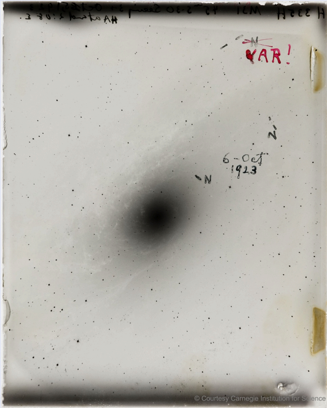
Edwin Hubble discovers the Universe. Créditos: Carnegie Institution for Science
