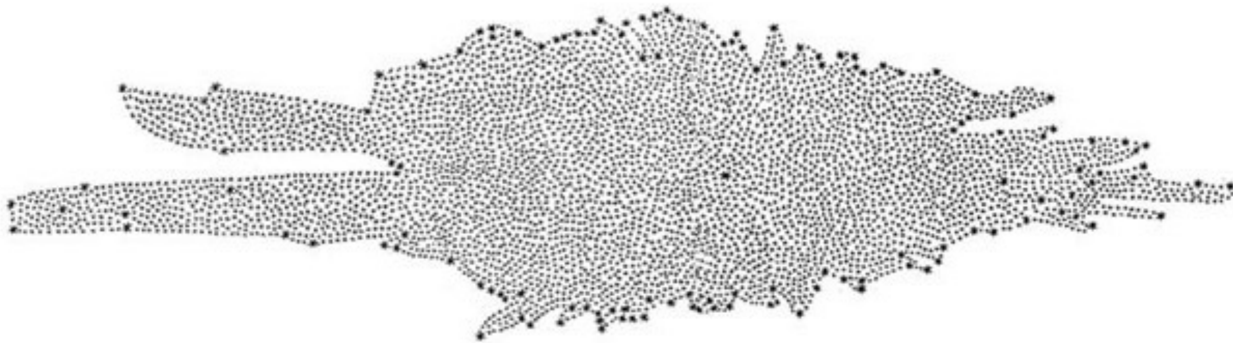
Figure 8.4: Herschel's map of the Milky Way from Herschel's 1785 publication showing his map of the Milky Way as derived from his counting of stars in various parts of the sky.
