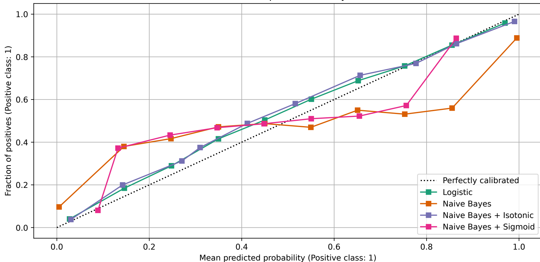
Logistic
