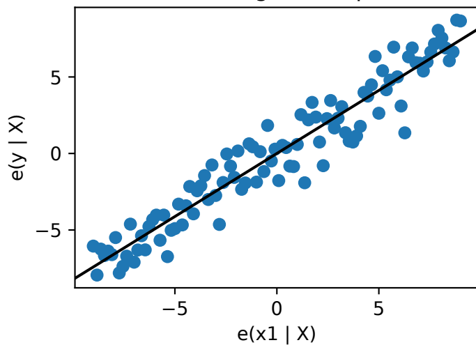
Partial regression plot
