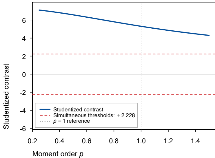
(b) Studentized contrast
