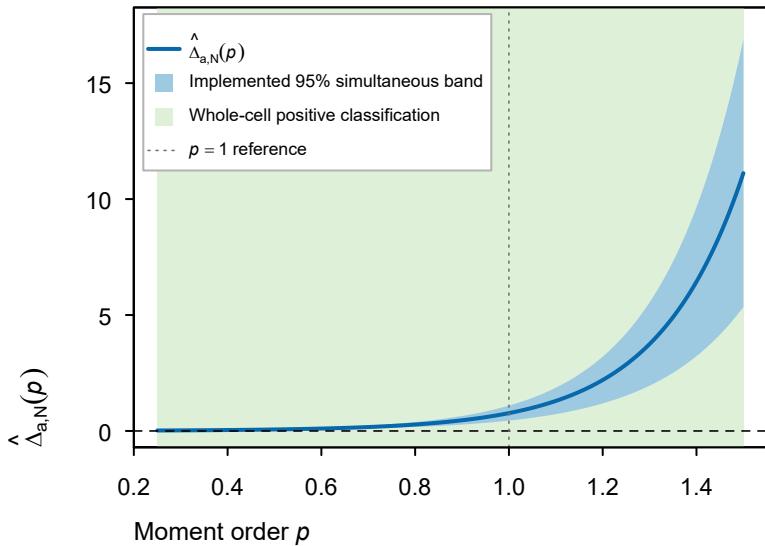
(a) Moment contrast
