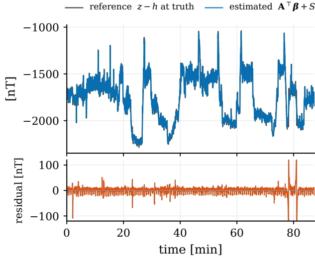
Fig. 5. Estimated \mathbf{A}^T \boldsymbol{\beta} + \mathbf{S} against the interference reference, and the residual (line 1007.06 Mag 4).
