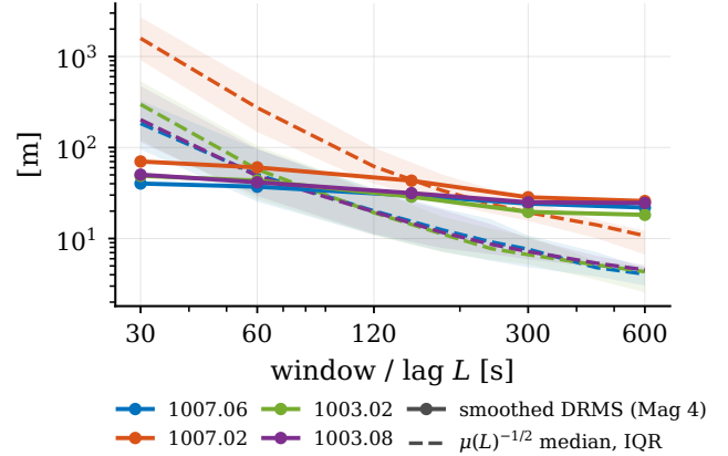
Fig. 10. Separability metric \mu(L)^{-1/2} of Eq. (20) (dashed, median and interquartile range over sliding windows) against the measured smoothed DRMS (solid, Mag 4), per line.
