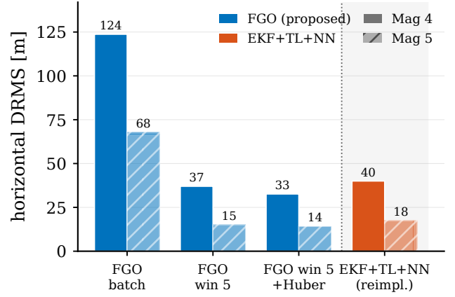
Fig. 9. Cold start on line 1007.06: NN-free fixed-lag window (left) versus the online EKF+TL+NN baseline (right).
