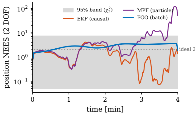
Fig. 11. Monte-Carlo position NEES versus time (EKF, marginalized particle filter, and batch FGO) with the 95 % \chi^2 band (ideal 2, dotted). NEES divides each estimator's error by its own reported covariance, so a lower curve means a more conservative filter, not a more accurate one; the EKF's larger errors over its larger causal covariance can plot below the more accurate smoother. Accuracy is compared by DRMS in the text.
