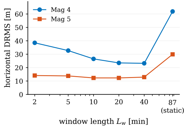
Fig. 8. Window length L_w versus horizontal DRMS on line 1007.06 (cold start).
