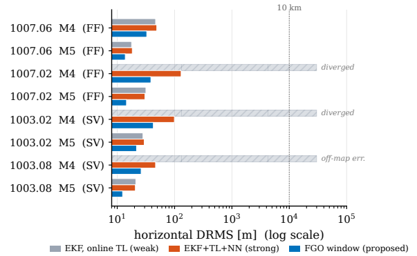
Fig. 10. Breadth study (Table III), log DRMS axis: online-TL EKF (gray), EKF+TL+NN (red), and the NN-free FGO window (blue). The MPF+TL particle filter diverges on every counted case and is omitted.
