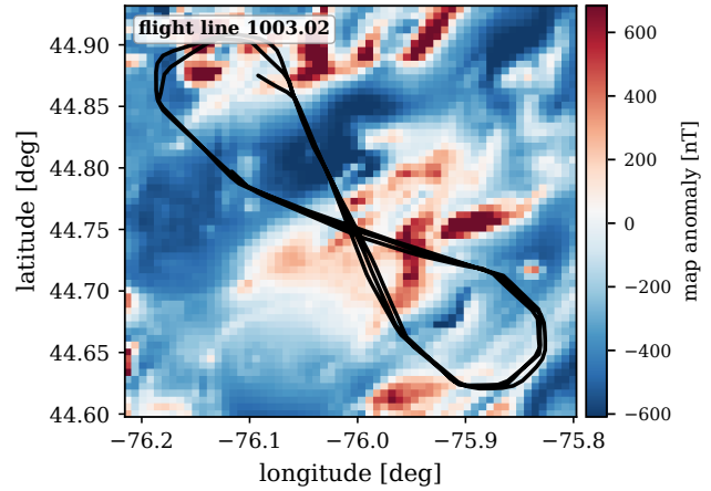
Fig. 6. Line 1003.02 over the Eastern anomaly map.
