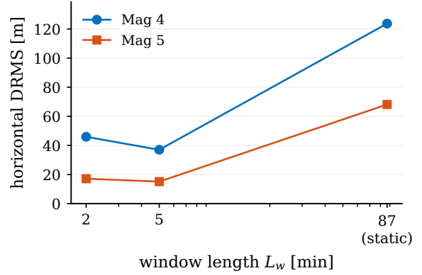
Fig. 8. Window length L_w versus horizontal DRMS on line 1007.06 (cold start).
