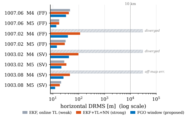
Fig. 10. Breadth study (Table III), log DRMS axis: online-TL EKF (gray), EKF+TL+NN (red), and the NN-free FGO window (blue).
