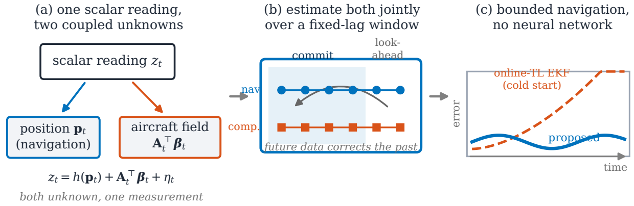
Fig. 1. Concept of the study: (a) one scalar reading couples aircraft position and aircraft-field compensation; (b) a fixed-lag factor graph estimates both jointly, letting later measurements correct earlier states; (c) bounded cold-start navigation, with no neural network.
