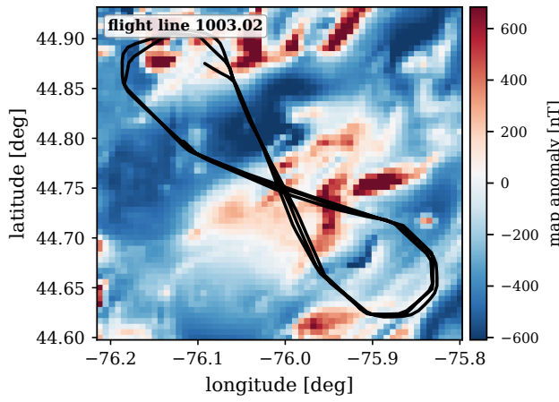
Fig. 6. Line 1003.02 over the Eastern anomaly map.
