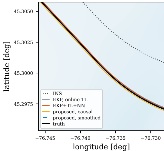
(b) zoom: the INS has drifted; aided paths hold the truth
