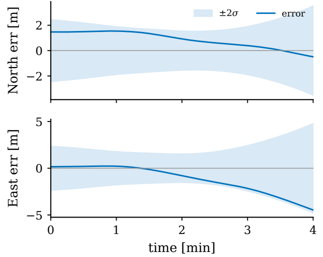
Fig. 12. North and East position error within the estimator \pm 2\sigma bands (representative simulated run of the batch FGO; the envelope is the smoother's own reported uncertainty, so this checks credibility, not accuracy). A calibrated Gaussian \pm 2\sigma band would be exceeded on \approx 5\% of epochs per axis; here the error approaches but never exits the band, the mildly conservative behaviour consistent with the ANEES below 2.
