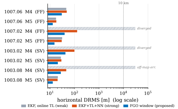
Fig. 12. Breadth study (Table III), log DRMS axis: online-TL EKF (gray), EKF+TL+NN (red), and the NN-free FGO window (blue). The MPF+TL particle filter is erratic at cold start (see text) and is omitted.
