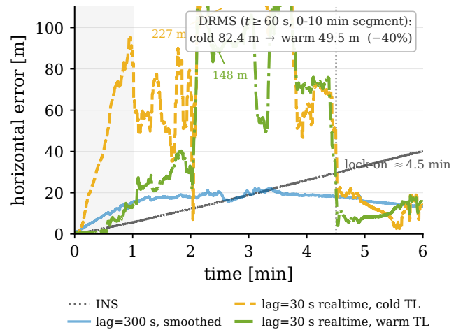
Fig. 7. First six minutes of the cold-start transient at a 30 s lag: a warm compensation prior roughly halves the penalty, but both runs lock on only at the strong map feature near four and a half minutes.
