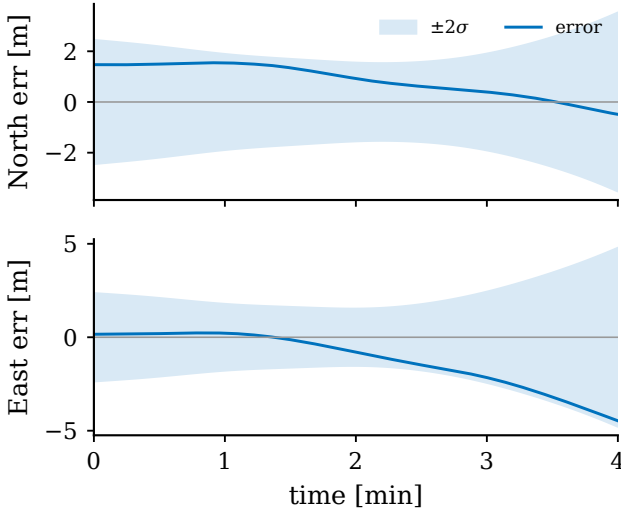
Fig. 14. North and East position error within the estimator \pm 2\sigma bands (representative simulated run of the batch FGO; the envelope is the smoother's own reported uncertainty, so this checks credibility, not accuracy). A calibrated Gaussian \pm 2\sigma band would be exceeded on \approx 5\% of epochs per axis; here the error approaches but never exits the band, the mildly conservative behaviour consistent with the ANEES below 2.
