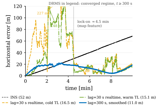
Fig. 16. Causal per-epoch estimates on the ten-minute segment: the 30 s-lag realtime error locks onto the map feature near four and a half minutes and converges toward the 300 s-lag smoothed estimate, far below free-inertial drift.
