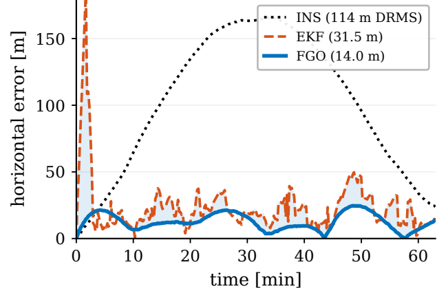
Fig. 9. Horizontal position error on line 1003.02: batch FGO, EKF, and free inertial (DRMS in the legend).
