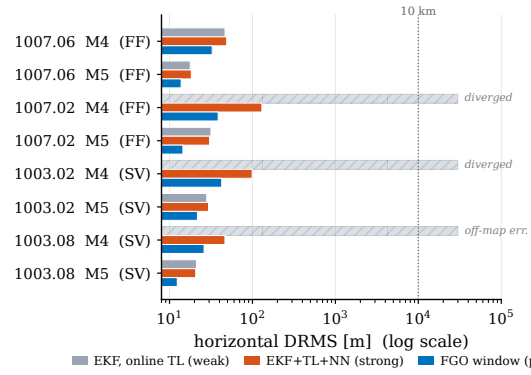
Fig. 10. Breadth study (Table III), log DRMS axis: online-TL EKF (gray), EKF+TL+NN (red), and the NN-free FGO window (blue). The MPF+TL particle filter diverges on every counted case and is omitted.
