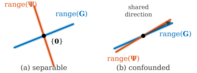
Fig. 5. Observability geometry (Proposition 1): position and compensation are separable when \text{range}(\mathbf{G}) and \text{range}(\Psi) meet only at the origin (left) and confounded when they share a direction (right).
