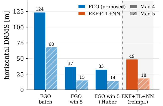
Fig. 9. Cold start on line 1007.06: NN-free fixed-lag window (left) versus the online EKF+TL+NN baseline (right).
