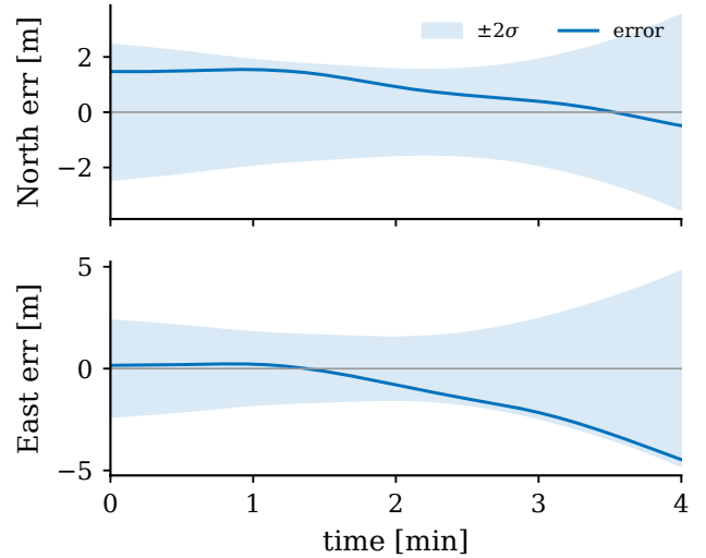
Fig. 12. North and East position error within the estimator \pm 2\sigma bands (representative simulated FGO run).
