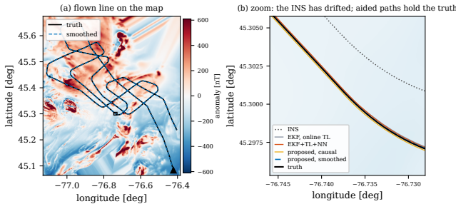
Fig. 4. Line 1007.06 Mag 4: (a) flown line with the zoom window; (b) late in the line, where the free-inertial drift peaks near 430 m, every aided path still holds the truth.
