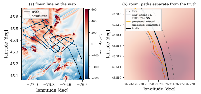
Fig. 4. Line 1007.06 Mag 4. (a) Flown line on the map, with the zoom window marked. (b) Zoom, in latitude/longitude, centred where the post-warm-up EKF error is largest: the estimated paths separate from the truth, with the committed estimate hugging it and the INS displaced to the east.
