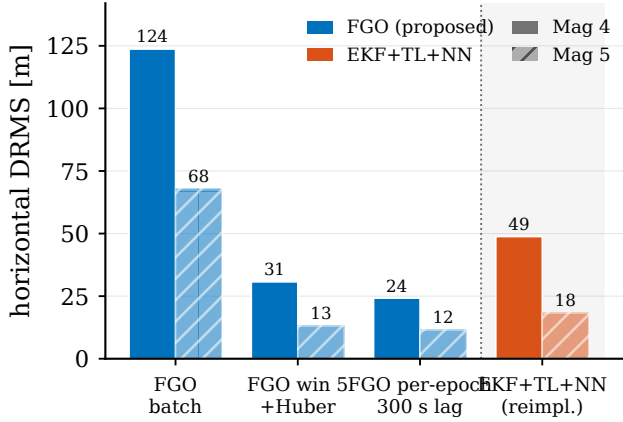
Fig. 11. Cold start on line 1007.06: the NN-free factor graph across the lag spectrum (left, per-epoch smoother highlighted) versus the online EKF+TL+NN baseline (right).
