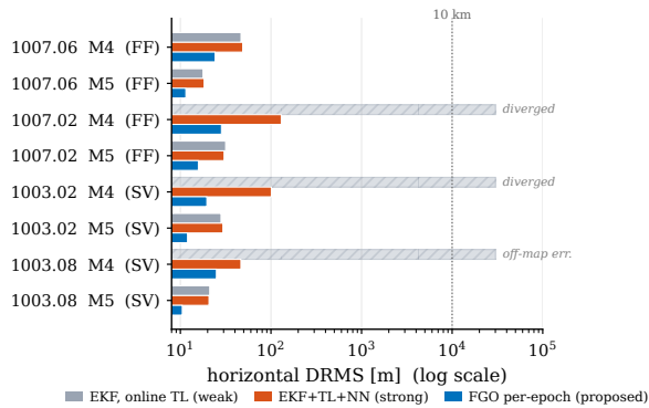
Fig. 12. Breadth study (Table III), log DRMS axis: online-TL EKF (gray), EKF+TL+NN (red), and the NN-free per-epoch FGO at a 300 s lag (blue). The sliding window is the intermediate lag and is tabulated rather than plotted; the MPF+TL particle filter is erratic at cold start (see text) and is omitted.
