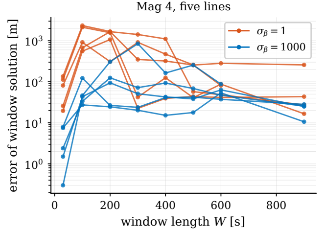
Fig. 17. Position error of the batch solution over the first W seconds of each Mag 4 line, from a zero compensation. At the nominal prior the solutions climb to kilometres over the middle window lengths; at the widened prior the excursion is absent on every line but the short calibration line 1006.08.
