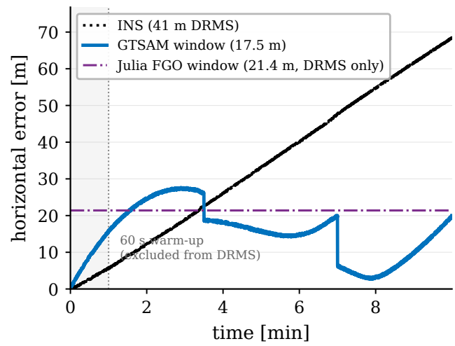
Fig. 15. Horizontal error of the independent GTSAM sliding window on the first ten-minute segment of line 1007.06, with the Julia smoother’s segment DRMS shown as a reference level (no Julia time series was exported for this run).
