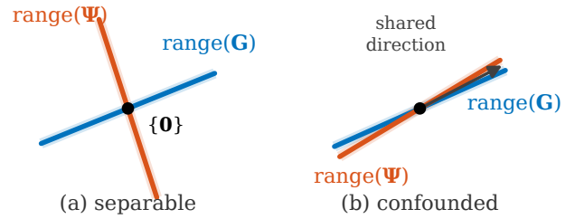
Fig. 5. Observability geometry (Proposition 1): position and compensation are separable when \text{range}(\mathbf{G}) and \text{range}(\boldsymbol{\Psi}) meet only at the origin (left) and confounded when they share a direction (right).
