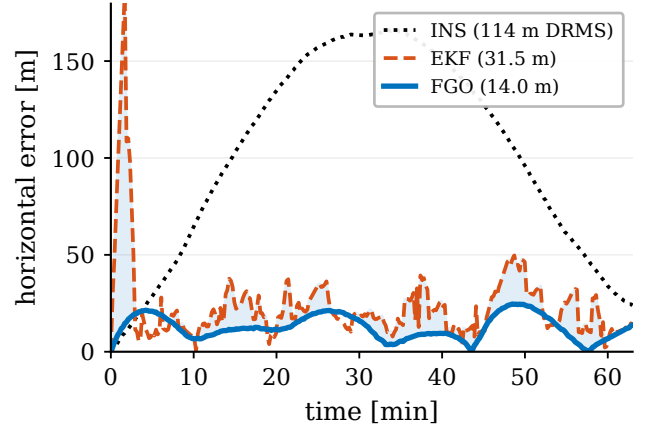
Fig. 9. Horizontal position error on line 1003.02: batch FGO, EKF, and free inertial (DRMS in the legend).
