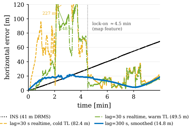
Fig. 16. Causal per-epoch estimates on the ten-minute segment: the 30 s-lag realtime error locks onto the map feature near four and a half minutes and settles close to the 300 s-lag smoothed estimate, far below free-inertial drift.
