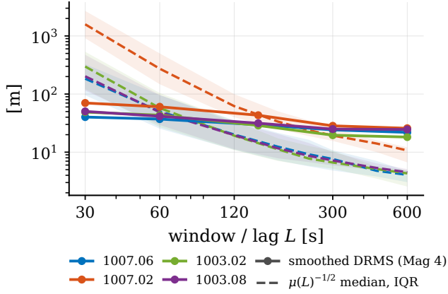
Fig. 10. Separability metric \mu^{-1/2} of Eq. (20) at window length L (dashed, median and interquartile range over sliding windows) against the measured smoothed DRMS at lag L (solid, Mag 4; the metric is sensor-independent), per line.
