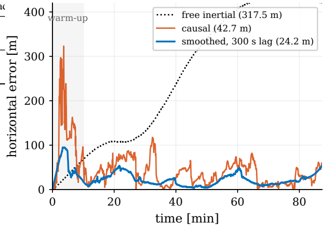
Fig. 7. Horizontal error, line 1007.06 Mag 4: the smoothed trace is the causal trace revised by the 300 s lag.
