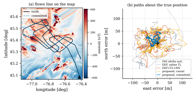
Fig. 4. Line 1007.06 Mag 4. (a) Flown line on the map; at this scale every bounded method overlays the truth. (b) The same paths in the north/east error plane about the true position, after the warm-up: the committed estimate stays tightest around the origin while the INS spirals out.
