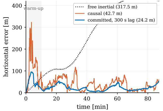
Fig. 7. Line 1007.06 Mag 4, cold start: horizontal error of the causal and the committed estimates against free-inertial drift. The committed trace is the causal trace revised by 300 s of look-ahead before each state is frozen.
