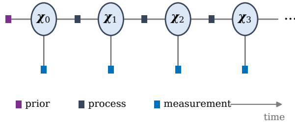
Fig. 2. Factor graph of a short trajectory. Circles are variable nodes, one per epoch; squares are factor nodes, each carrying one piece of information. The unary prior anchors the first state, binary process factors link consecutive states, and a unary measurement factor hangs from every state. A factor depends only on the variables it is joined to, which is what makes the problem sparse.
