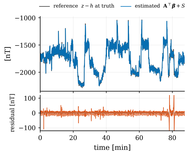
Fig. 5. What the compensation chain learned (Mag 4): the estimated \mathbf{A}^T \beta + S overlays the interference reference; the residual is tens of nanotesla.
