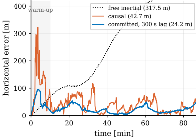
Fig. 6. Line 1007.06 Mag 4, cold start: horizontal error of the causal and the committed estimates against free-inertial drift. The committed trace is the causal trace revised by 300 s of look-ahead before each state is frozen.
