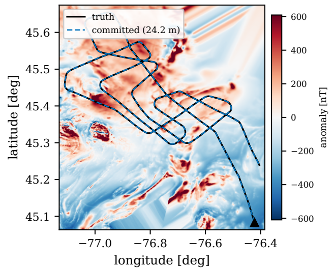
Fig. 4. Line 1007.06: committed estimate against truth on the anomaly map.
