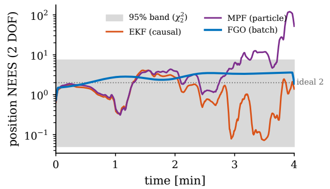
Fig. 11. Monte-Carlo position NEES versus time (EKF, marginalized particle filter, and batch FGO) with the 95 % \chi^2 band (ideal 2, dotted). NEES divides each estimator's error by its own reported covariance, so a lower curve means a more conservative filter, not a more accurate one; the EKF's larger errors over its larger causal covariance can plot below the more accurate smoother. Accuracy is compared by DRMS in the text.
