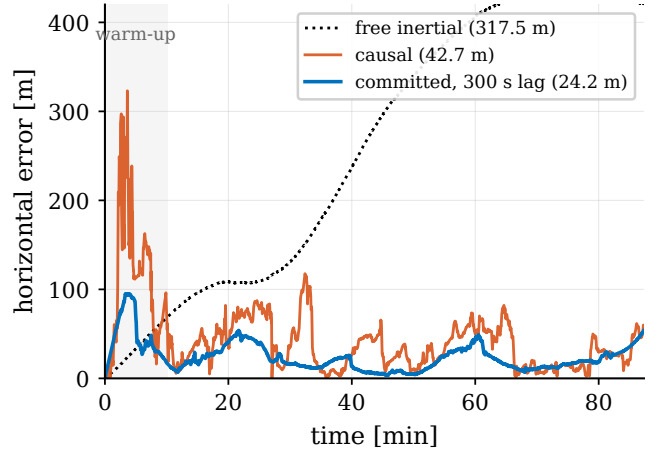
Fig. 8. Line 1007.06 Mag 4, cold start: horizontal error of the causal and the committed estimates against free-inertial drift. The committed trace is the causal trace revised by 300 s of look-ahead before each state is frozen.
