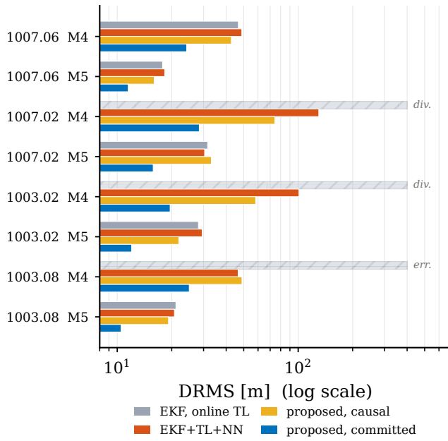
Fig. 9. Breadth comparison of Table IV on a log axis.
