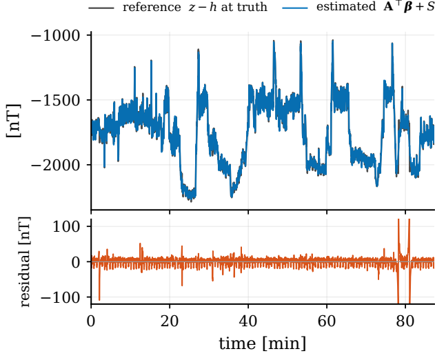
Fig. 6. What the compensation chain learned (Mag 4): the estimated \mathbf{A}^\top \boldsymbol{\beta} + S overlays the interference reference; the residual is tens of nanotesla.
