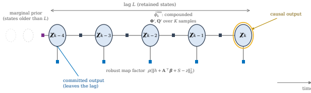
Fig. 3. The graph the smoother maintains, exactly as implemented. Circles are the joint states at the 1 Hz cadence; binary factors carry the transition and process noise compounded over the K intervening samples; a robust map factor hangs from every state; everything older than the lag is summarized by the marginal prior on the oldest retained state. The causal output is read at the newest state, the committed output where states leave the lag.
