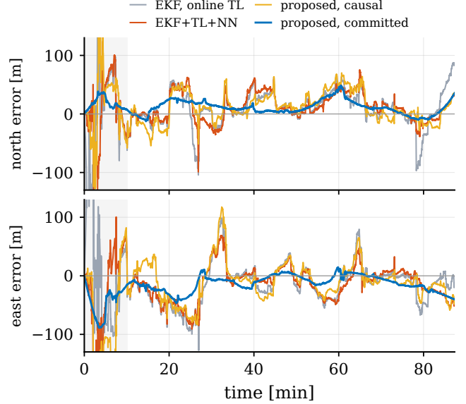
Fig. 7. North and east error histories of the compared methods on line 1007.06 Mag 4. The EKF+TL+NN trace is a fresh run of the seed-sensitive filter (40.0 m on this run, against the fixed reference run of Table III).
