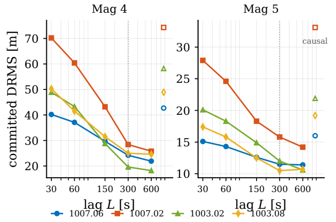
Fig. 10. Committed DRMS against lag (Table V); open markers show the lag-independent causal error.
