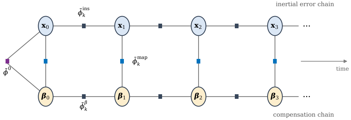
Fig. 4. Factor graph of the joint problem. The inertial error chain (top) and the compensation chain (bottom) evolve under their own process factors and are coupled at every epoch by the scalar map factor, which is the only place the two unknowns meet, and the reason they must be estimated together.
