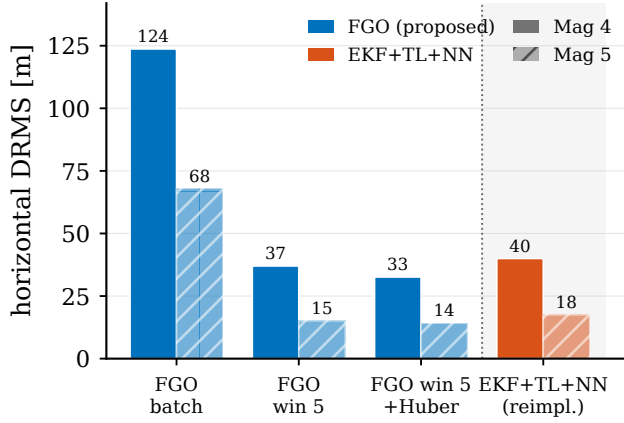
Fig. 9. Cold start on line 1007.06: NN-free fixed-lag window (left) versus the reimplemented EKF+TL+NN (right).
