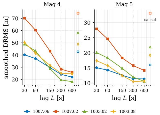
Fig. 9. Smoothed DRMS against lag (Table V); open markers show the lag-independent causal error.
