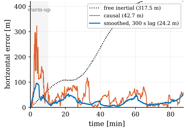
Fig. 7. Line 1007.06 Mag 4, cold start: horizontal error of the causal and the smoothed estimates against free-inertial drift. The smoothed trace is the causal trace revised by 300 s of look-ahead before each state is frozen.
