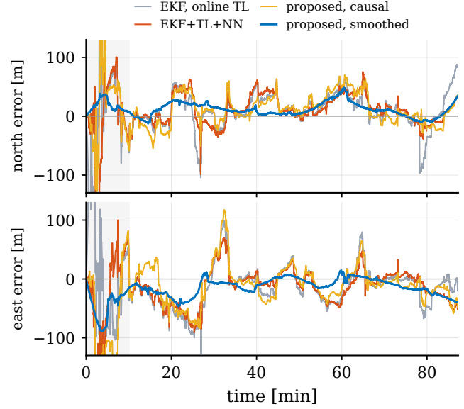
Fig. 6. North and east error histories, line 1007.06 Mag 4. The EKF+TL+NN is a fresh run (40.0 m here; ten-seed median 43.8 m).
