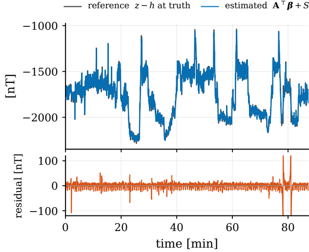
Fig. 5. Estimated \mathbf{A}^T \boldsymbol{\beta} + S against the interference reference, and the residual (line 1007.06 Mag 4).
